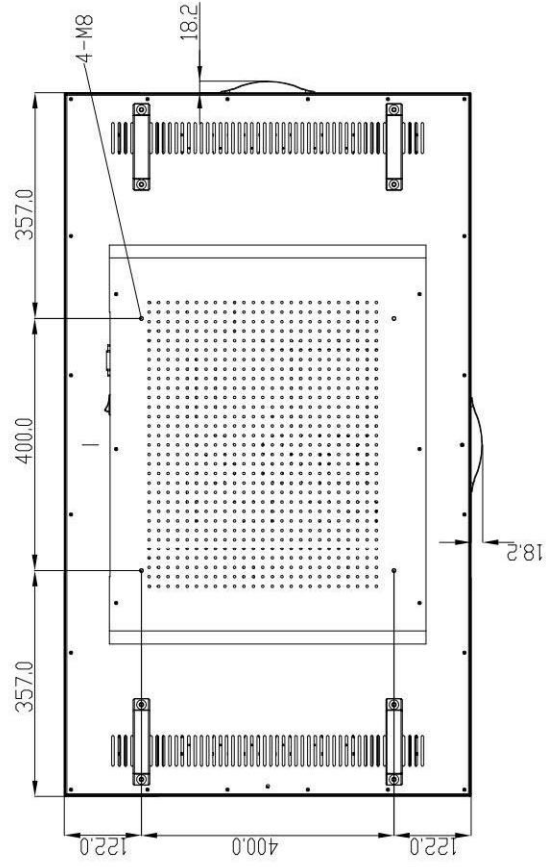
49 inch Dimensions
